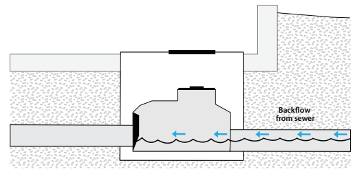
Install & Maintain a Backwater Valve
