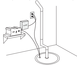
Test Sump Pump & Install Backup Power
