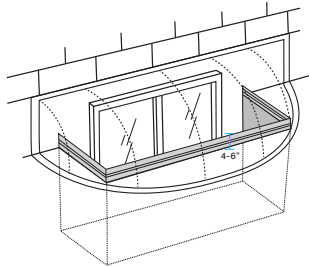
Install Window Wells & Covers
